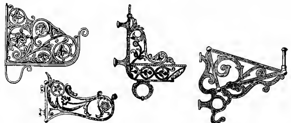
Figs. 3767-3770. CAST BRACKET-ENDS FOR BASKET-RACKS.
